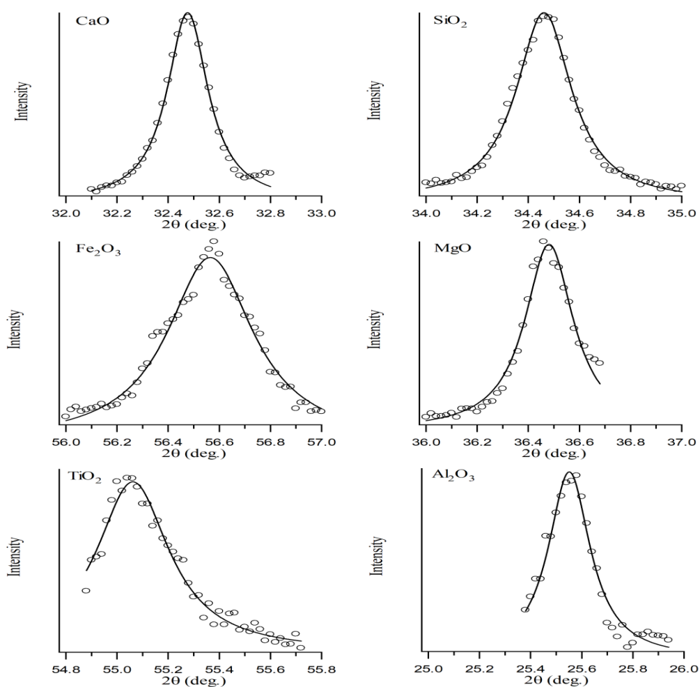
Figure 3. The comparison of the XRD data (circles) and calculated the best fit of Lorentzian function (solid lines) for the bio-solar gemstone
